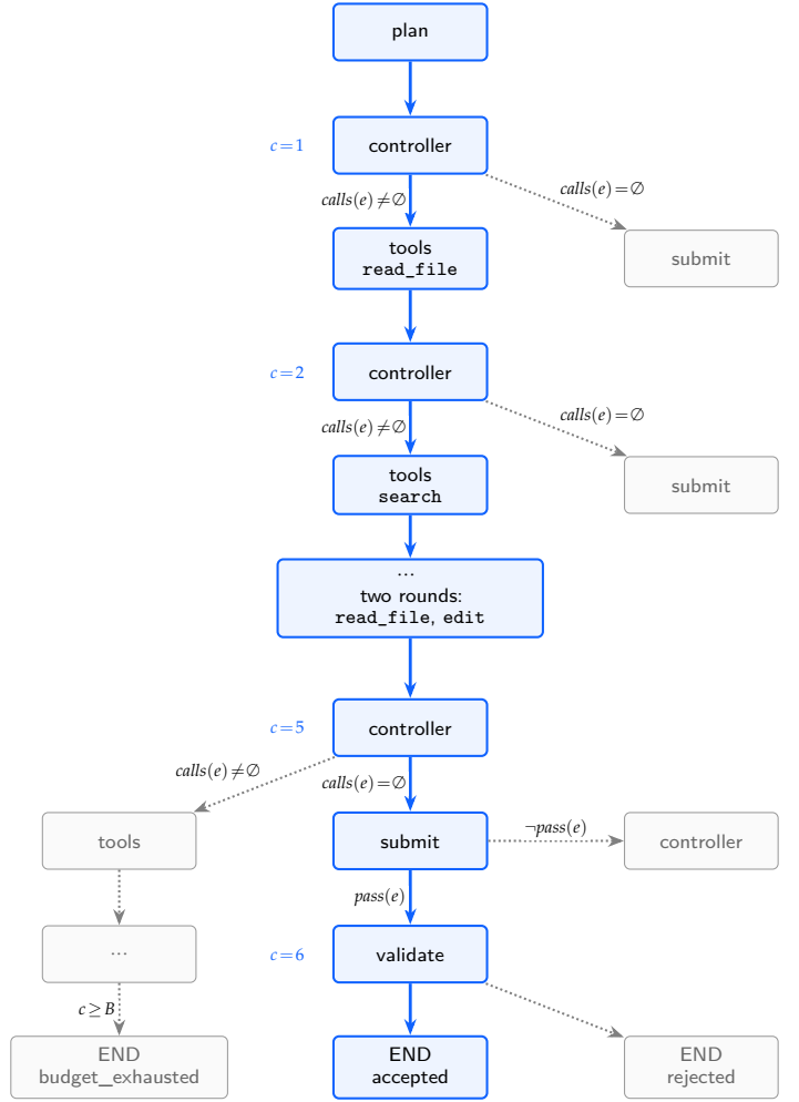
Figure 2: A fragment of the planning agent’s computation tree around run bc284c6b. Blue nodes and edges show the recorded trajectory; the \dots node omits two controller and tool rounds. Dotted grey branches are continuations the guards permit under other replies or check results; the grey \dots omits further rounds. c is the number of model calls completed on reaching a node, derived from the log and the set actions. No probabilities are implied.
