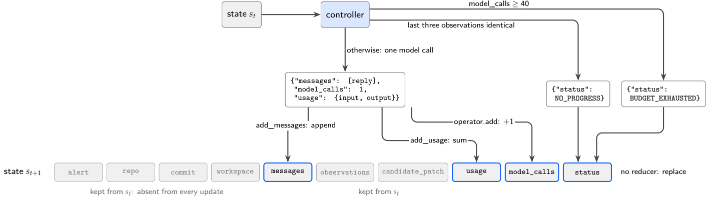
Figure 4: The controller’s three return sites against the loop’s ten-key record. The guard on each edge selects the path. The path that calls the model returns three keys, and each of the two paths that stop the run returns one. An arrow into a key names the reducer the runtime applies to it. status has no reducer, so the returned value replaces the stored one. The six keys without an arrow are absent from every update and keep their values from s_t .
