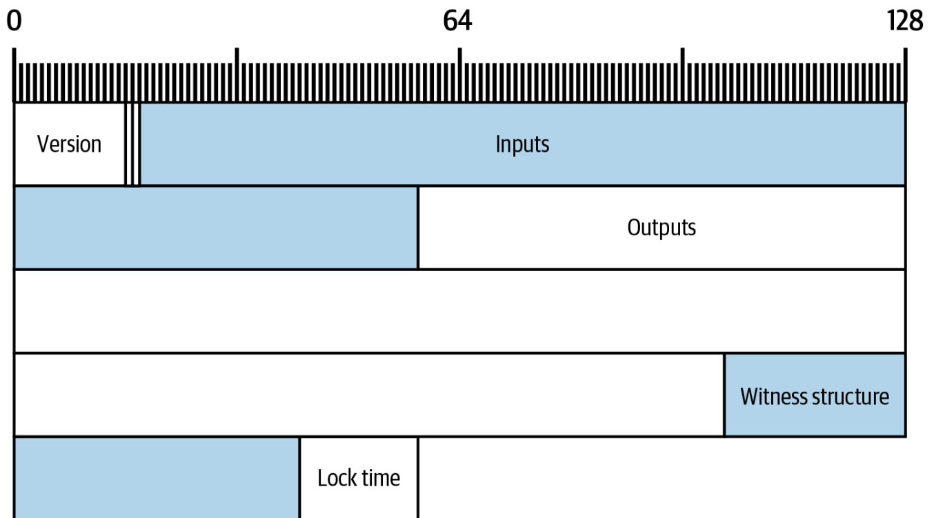
Figure 36. Ramani ya baiti ya muamala wa Alice.
