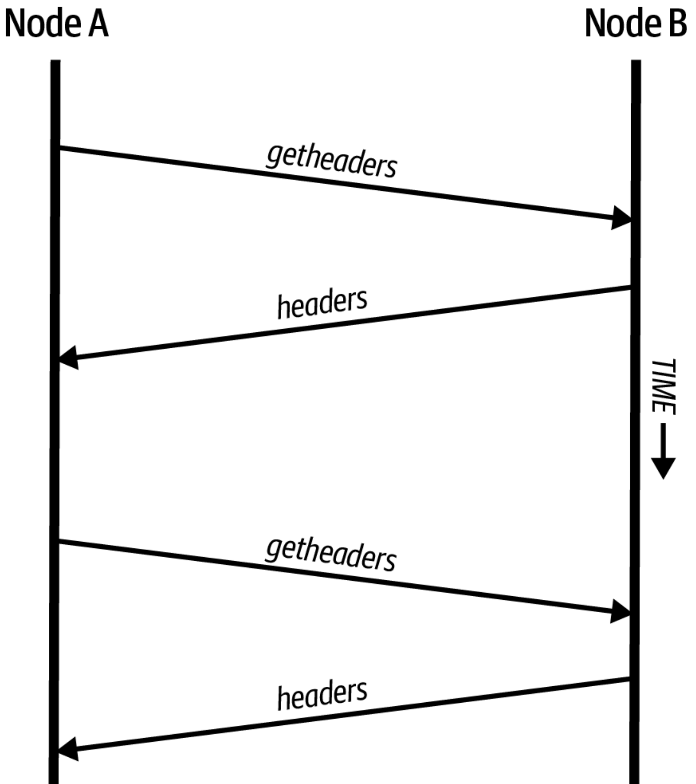
Figure 51. Mteja mwepesi akisawazisha vichwa vya vitalu.
