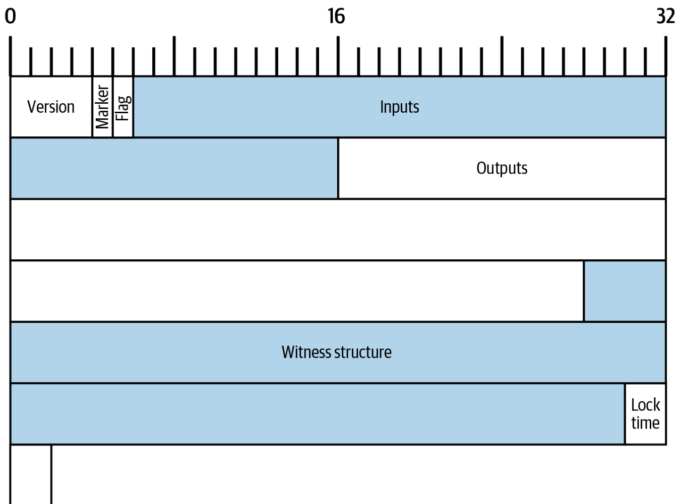
Figure 31. Ramani ya baiti ya muamala wa Alice.
