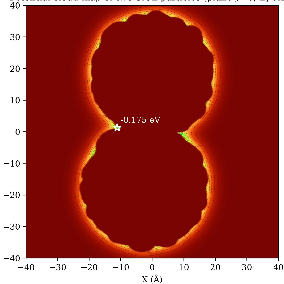
Potential cloud-map of two SiO 2 particles (plane y=0 ; LJ only)
