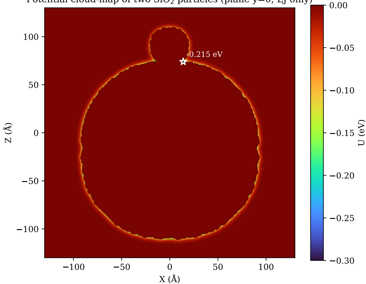
Potential cloud-map of two \text{SiO}_2 particles (plane y=0 ; LJ only)
