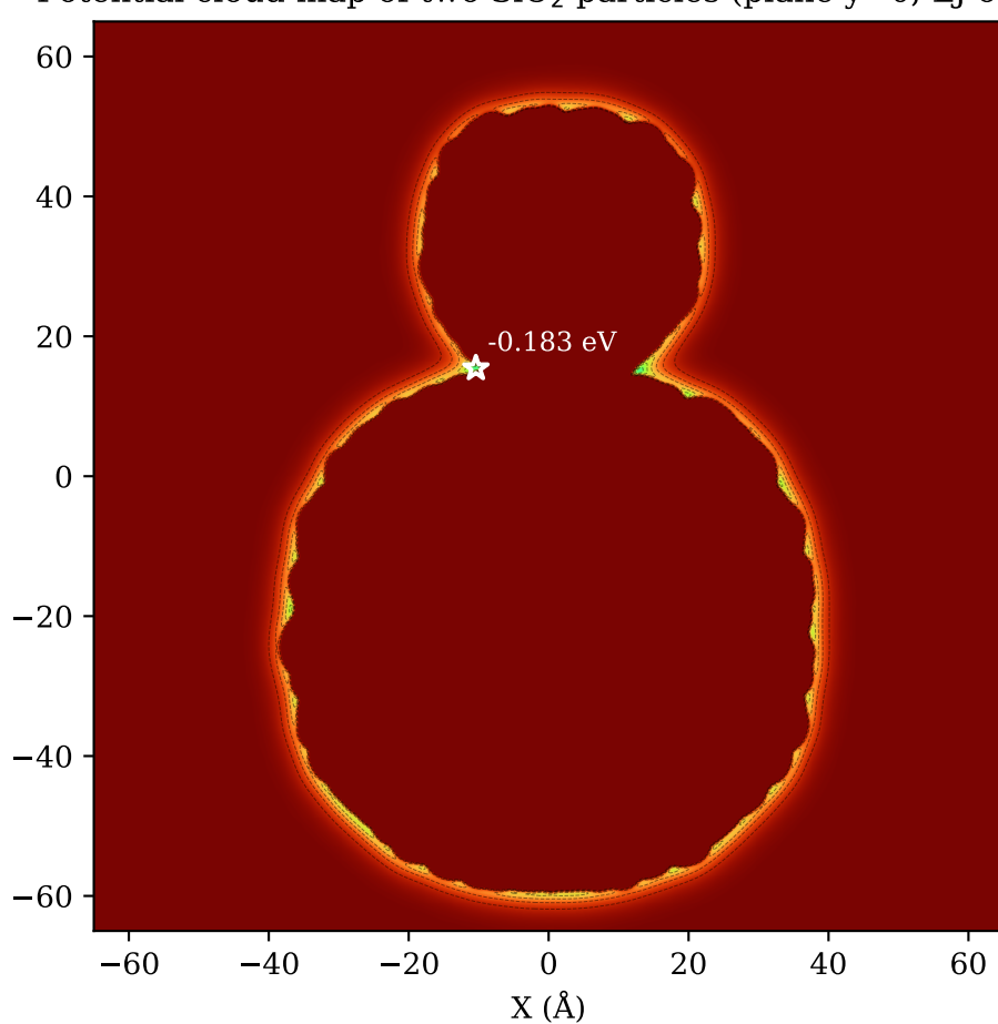
Potential cloud-map of two \text{SiO}_2 particles (plane y=0 ; LJ only)
