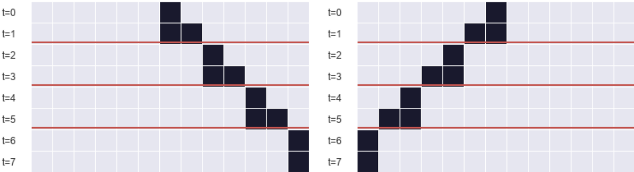
Figure 6. Moving oscillator (glider) -- period T=2, speed 1 rule_20 (drift +2) rule_6 (drift -2)
