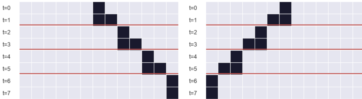
Figure 6. Moving oscillator (glider) -- period T=2 , speed 1
