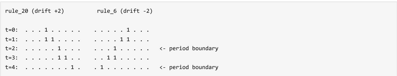
Figure 6. Moving oscillator (glider) -- period T=2, speed 1.
