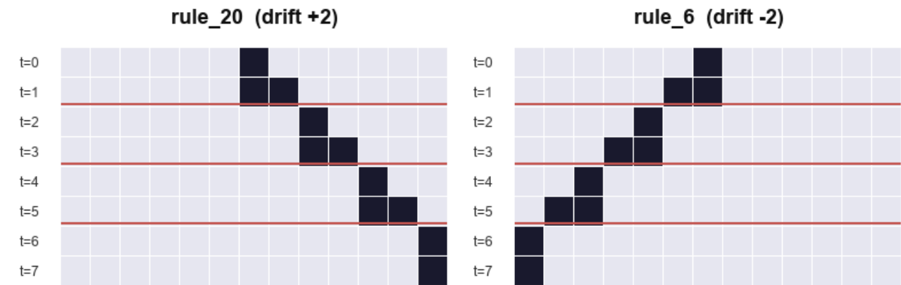
Figure 6. Moving oscillator (glider) -- period T=2, speed 1
