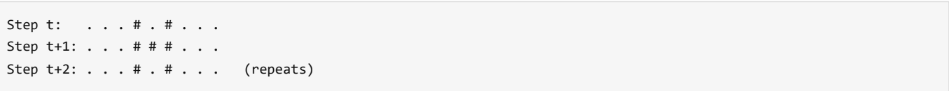
Figure 4. rule_108 period-2 oscillator motif.
