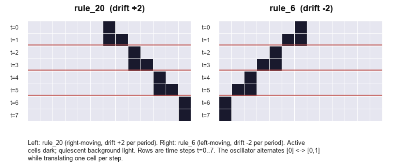
Figure 6. Moving oscillator (glider) -- period T=2, speed 1
