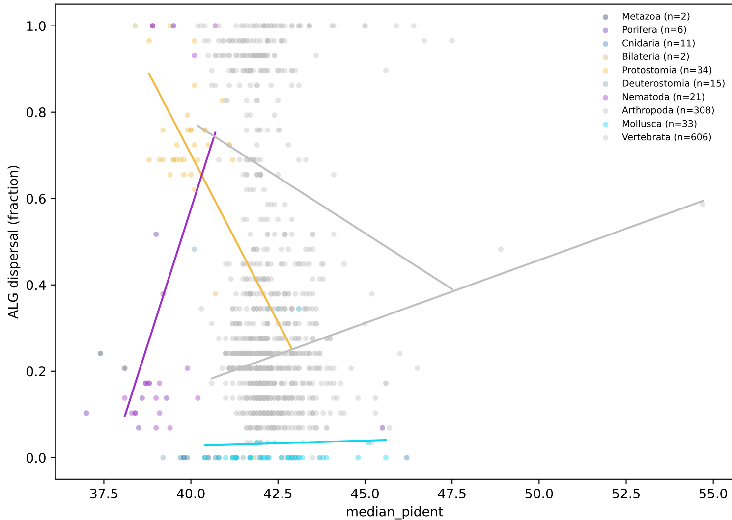
Protein divergence vs ALG dispersal
