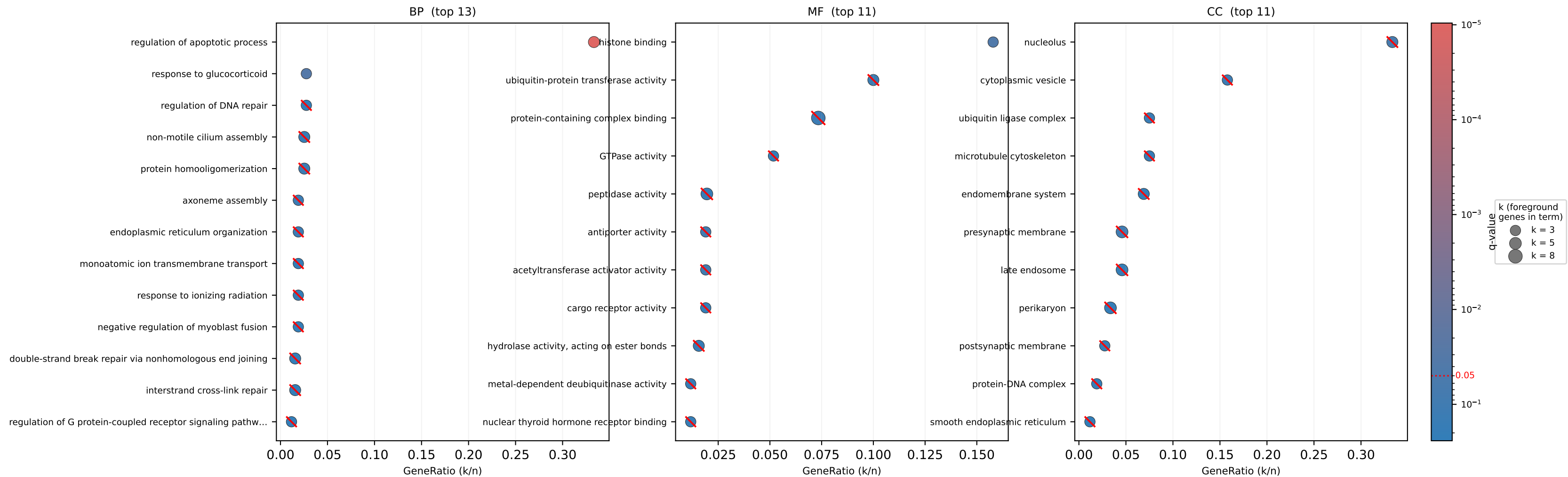
Platyhelminthes — top GO enrichments per namespace (fold ≥ 3×, k ≥ 3)
