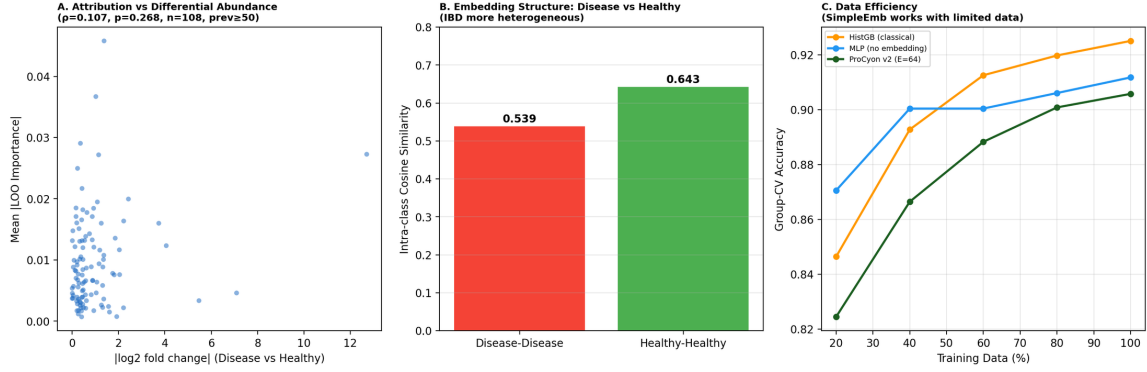
Figure 12: Attribution biology and embedding structure. (A) LOO importance vs. |\log_2 fold change| scatter (prevalence \geq 50 ). (B) Intra-class cosine similarity: disease vs. healthy. (C) Data efficiency comparison.
