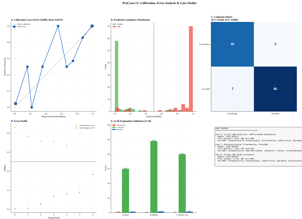
Figure 13: Calibration, error analysis, and case studies. (A) Calibration curve (ECE=0.05, Brier=0.056). (B) Prediction confidence distribution. (C) Confusion matrix. (D) Error profile: false positives vs. false negatives. (E) LLM explanation validation summary. (F) Case study overview.
