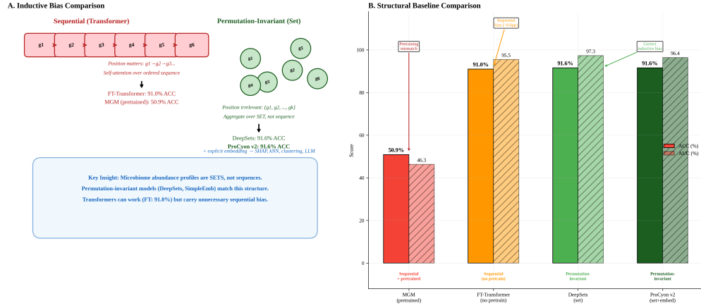
Figure 5: Inductive bias comparison. (A) Sequential (Transformer) vs. permutation-invariant (Set) inductive biases with corresponding model performance. (B) Structural baseline accuracy and AUROC comparison.
