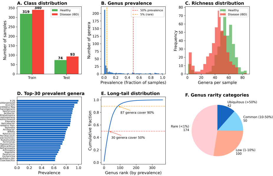
Figure 2: Dataset statistics for clean_2538. (A) Class distribution. (B) Genus prevalence distribution. (C) Richness distribution. (D) Top-30 most prevalent genera. (E) Long-tail cumulative distribution. (F) Genus rarity categories.
