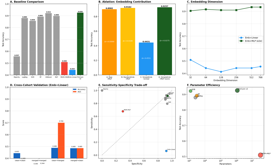
Figure 4: Comprehensive comparison analysis. (A) Baseline accuracy comparison. (B) Ablation: embedding contribution. (C) Embedding dimension sweep. (D) Cross-dataset transfer. (E) Sensitivity-specificity trade-off. (F) Parameter efficiency.
