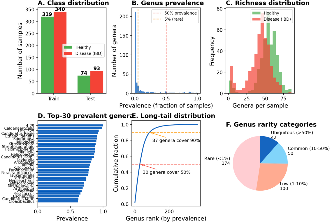
Figure 2: Dataset statistics for clean_2538. (A) Class distribution. (B) Genus prevalence distribution. (C) Richness distribution. (D) Top-30 most prevalent genera. (E) Long-tail cumulative distribution. (F) Genus rarity categories.
