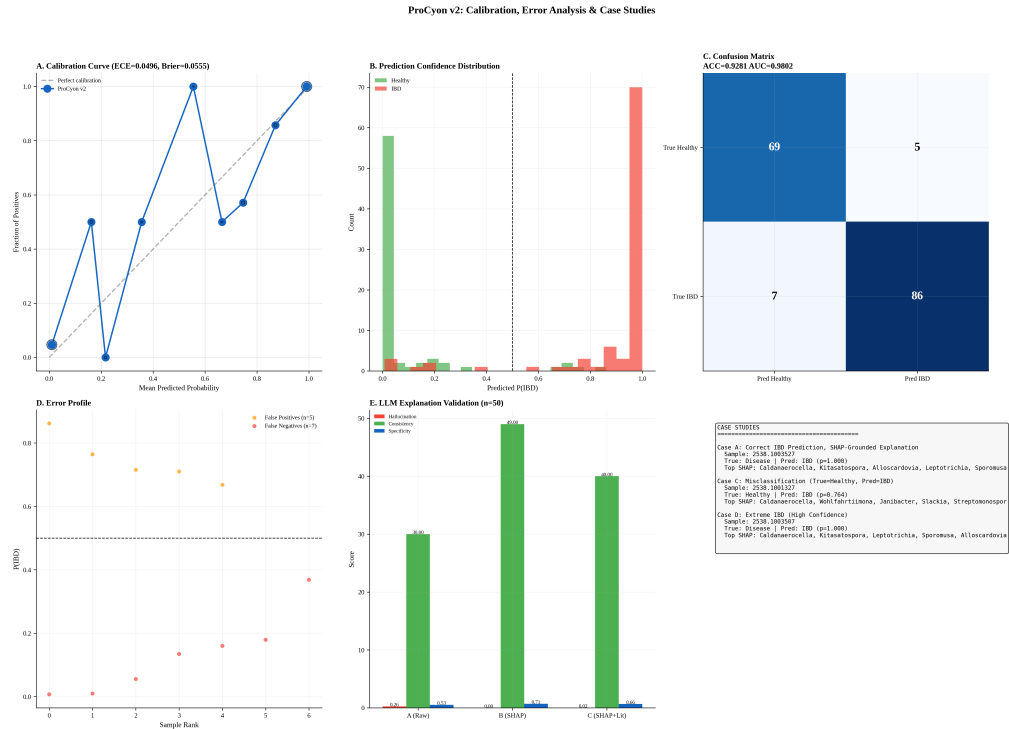
Figure 13: Calibration, error analysis, and case studies. (A) Calibration curve (ECE=0.05, Brier=0.056). (B) Prediction confidence distribution. (C) Confusion matrix. (D) Error profile: false positives vs. false negatives. (E) LLM explanation validation summary. (F) Case study overview.
