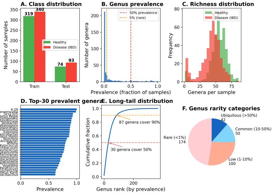
Figure 2: Dataset statistics for clean_2538. (A) Class distribution. (B) Genus prevalence distribution. (C) Richness distribution. (D) Top-30 most prevalent genera. (E) Long-tail cumulative distribution. (F) Genus rarity categories.
