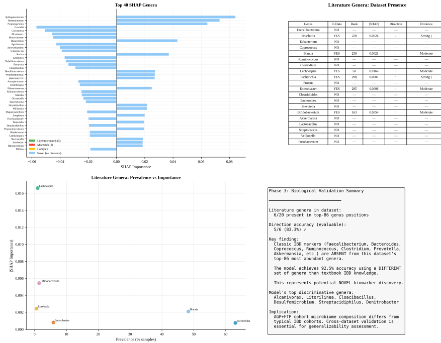
Figure 9: Biological validation against literature. Direction agreement between model LOO attribution and 20 literature-curated Crohn's disease-associated genera from Paidimarri et al. (2024).
