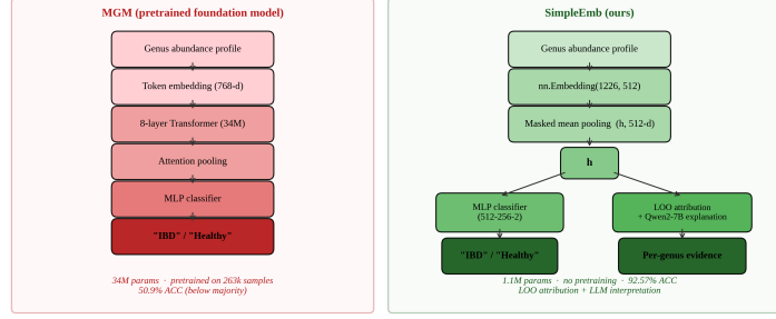
Figure 1: Architecture comparison. SimpleEmb (right) maps each present genus to a learned 512-d embedding, summarizes the profile by masked mean pooling, and predicts IBD; the same embedding space powers leave-one-out (LOO) attribution, verbalized by a frozen Qwen2-7B. MGM (left) is a 34M-parameter pretrained Transformer that reaches only 50.9% accuracy here.
