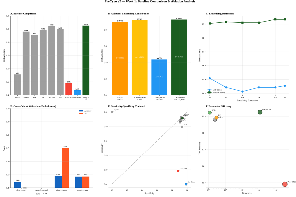
Figure 4: Comprehensive comparison analysis. (A) Baseline accuracy comparison. (B) Ablation: embedding contribution. (C) Embedding dimension sweep. (D) Cross-dataset transfer. (E) Sensitivity-specificity trade-off. (F) Parameter efficiency.
