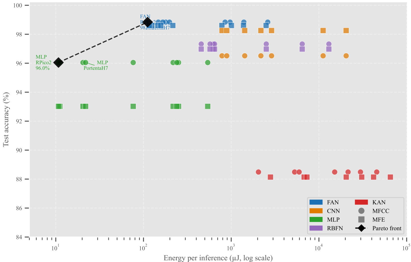
Figure 6 — Embedded Pareto Frontier: Test Accuracy vs. Energy per Inference
