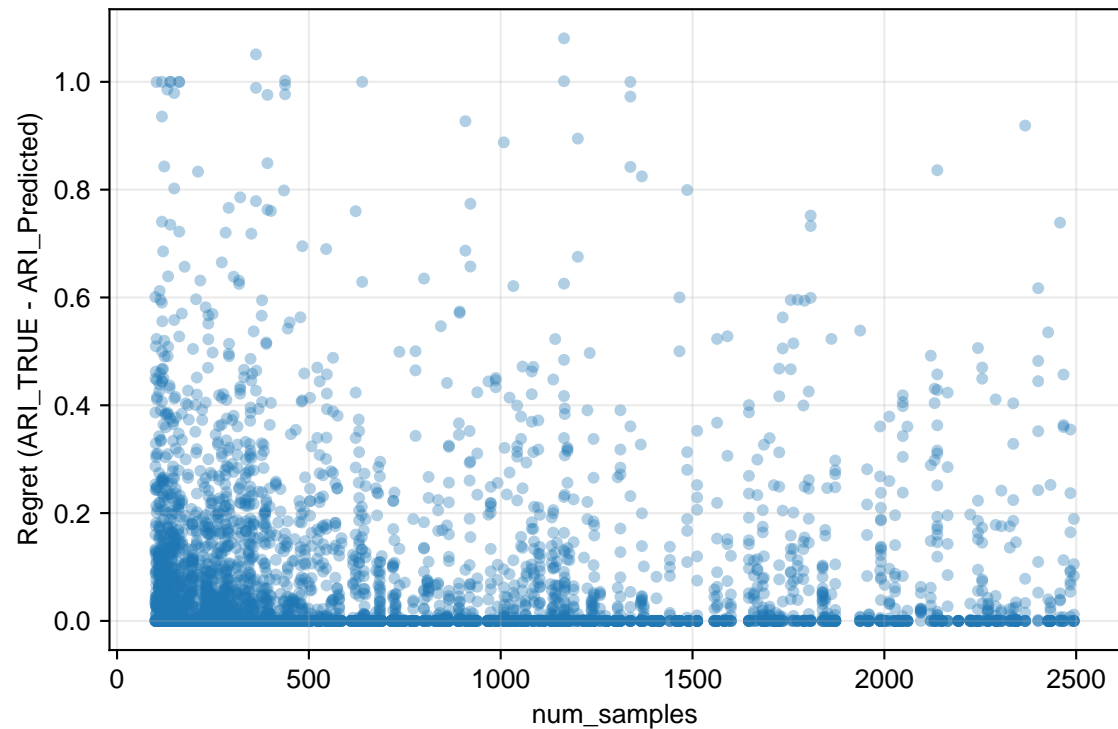
Regret vs #Samples (n) Spearman \rho = -0.126
