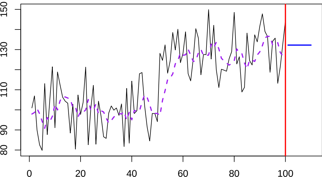
SES with \alpha=0.242
