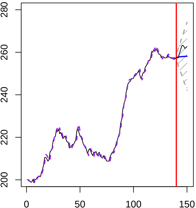
Parametric prediction interval
