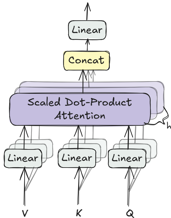
Multi-Head Attention
