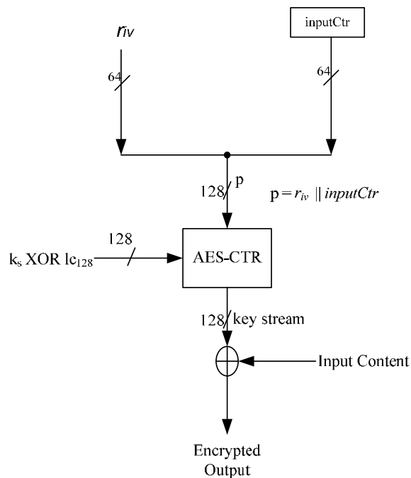
Figure 3-2. HDCCP Cipher Structure
