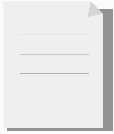
Textual modality
