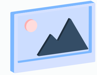
Visual modality
