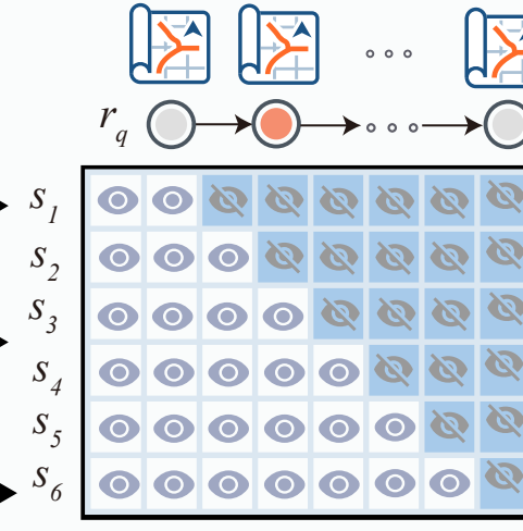
Causal masked Transformer
