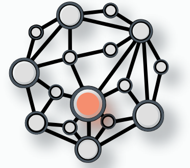
Knowledge graph
