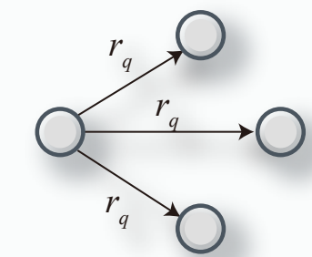
Query association
