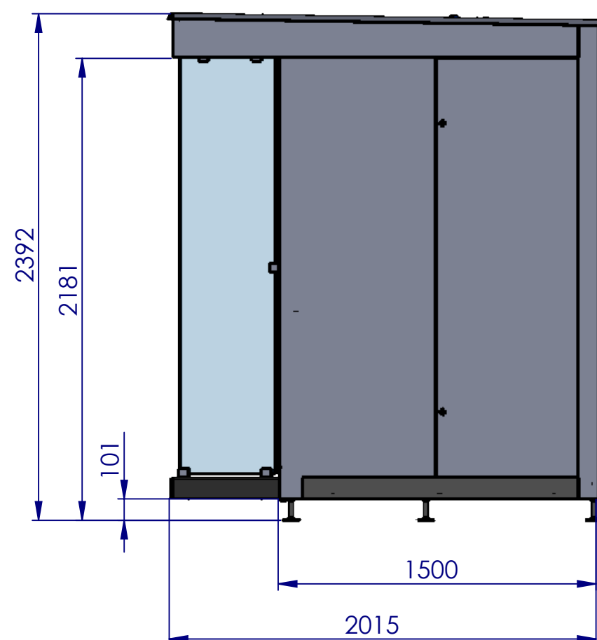
RIGHT VIEW
