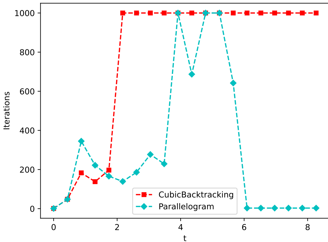
Inner iterations
