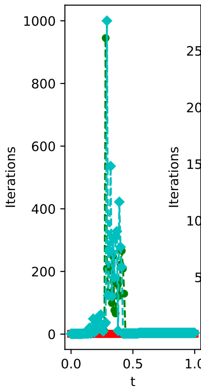
Outer iterations
