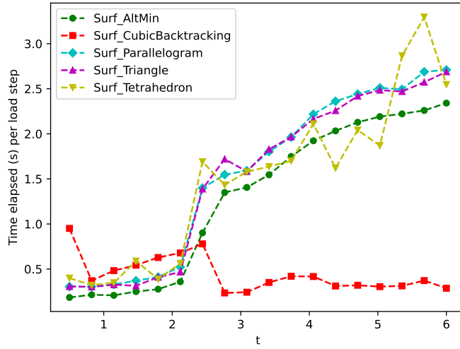
Figure 5: Wall clock time for solving the surfing example for all five methods.
