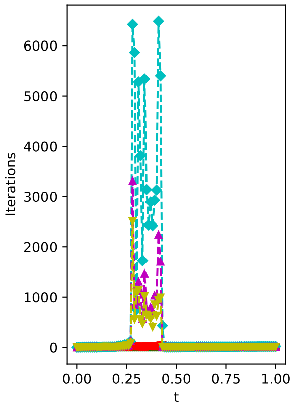
Inner iterations
