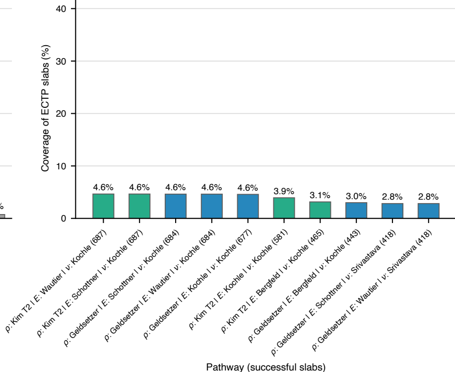
Density Method
