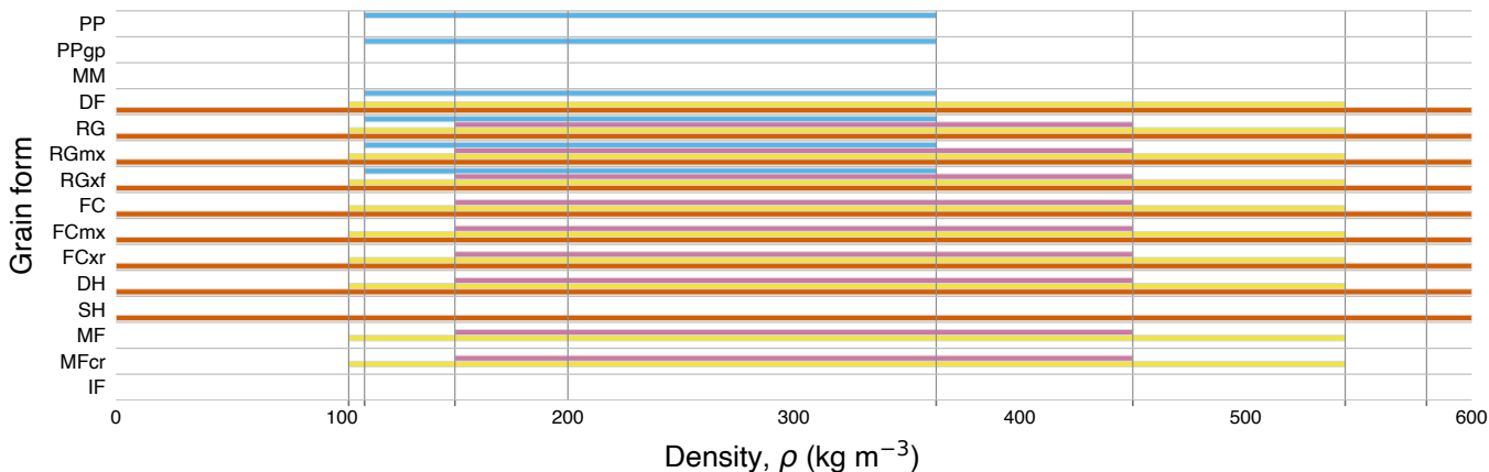
(b) Elastic modulus methods: support narrows by density and grain form
