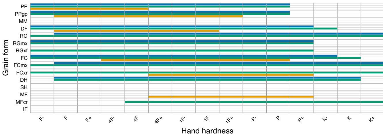
(a) Density methods: support depends on grain form and hand hardness
