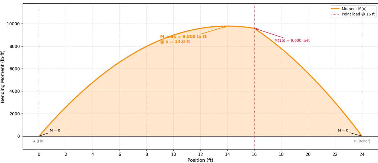
Moment Diagram - 24 ft Simply Supported Beam
