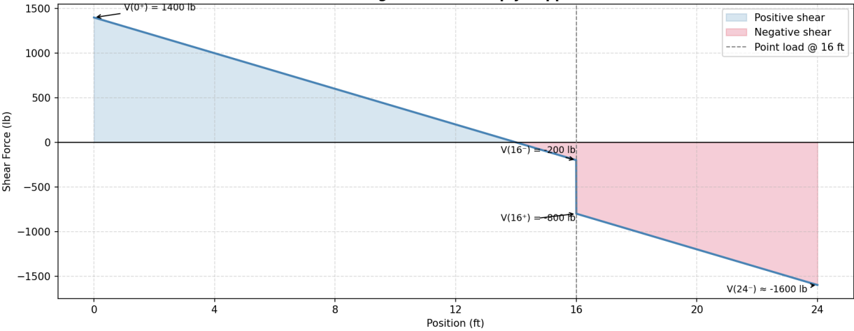
Shear Force Diagram - 24 ft Simply Supported Beam
