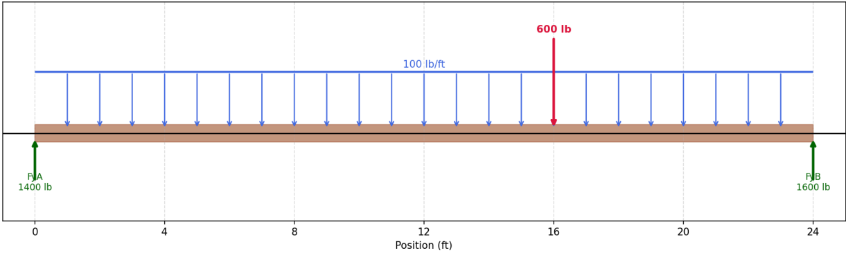
Load Diagram - 24 ft Simply Supported Beam
