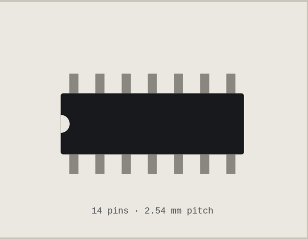
DIP Dual In-line Package
