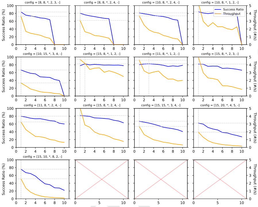
Fig. 11. Independent Parameter: #ASS of REIFY°. This plot shows that #ASS is another major parameter influencing the scalability and performance of REIFY°, alongside #BBL. This is expected, as an increase in assignments per basic block raises the number of constraints by at least the number of basic blocks. For any configuration, once the number of assignments exceeds a certain threshold, the success ratio drops sharply. This is because the additional assignments generate a dense set of constraints over a limited set of variables, increasing the likelihood of being unsatisfiable. According to it, choosing 2–5 assignments per basic block leads to a better balance among all evaluated configurations.
