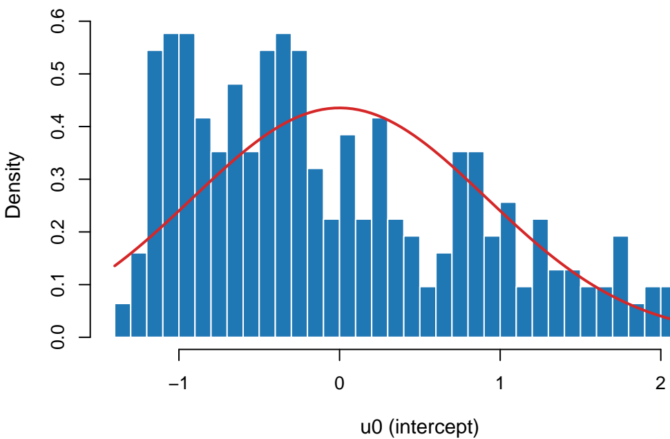
Random intercepts
