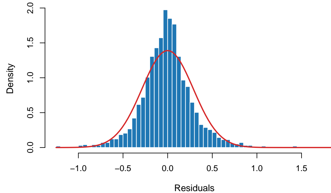
Residual distribution
