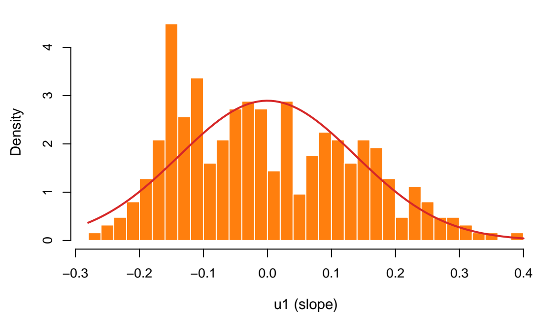
Random slopes
