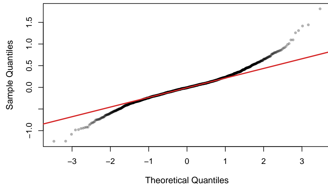
Normal Q-Q (residuals)
