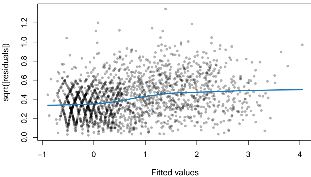
Scale-Location
