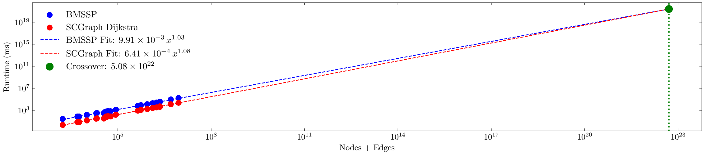
BMSSP vs SCGraph Dijkstra – Estimated Square Gridgraph Crossover Point
