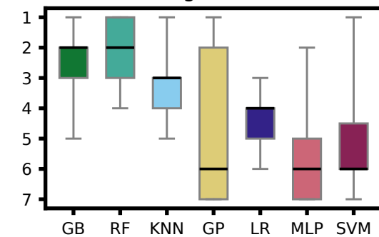
Regression
