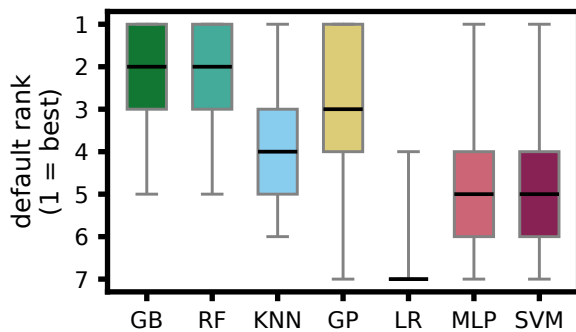
Classification
