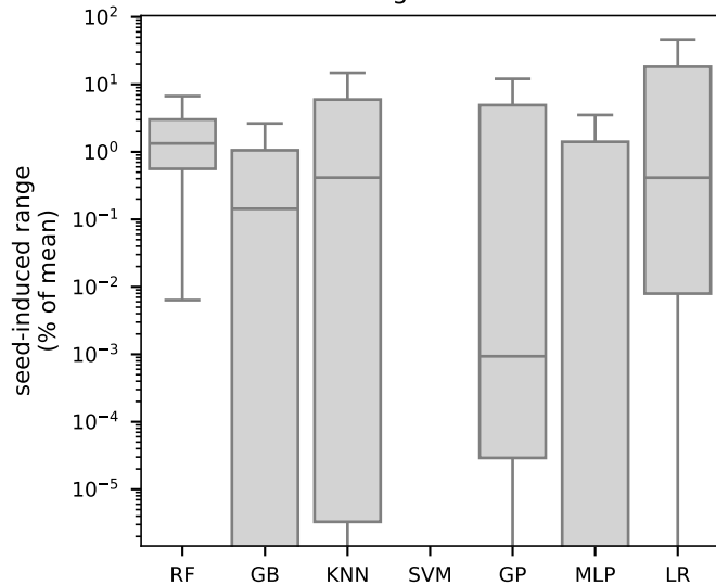
Regression
