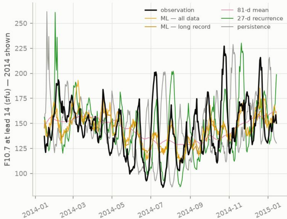
Observed vs modeled F10.7
