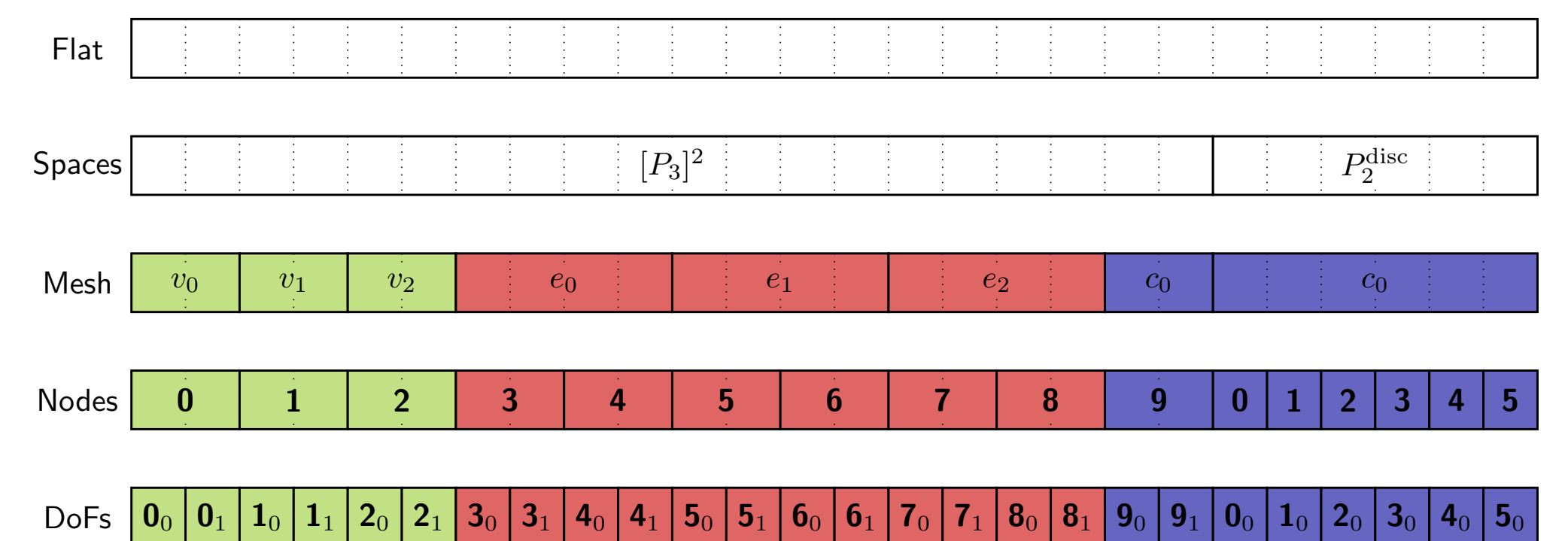
Figure 4: Different views of a possible data layout for a one-cell mesh of the finite element pair in fig. 3.
