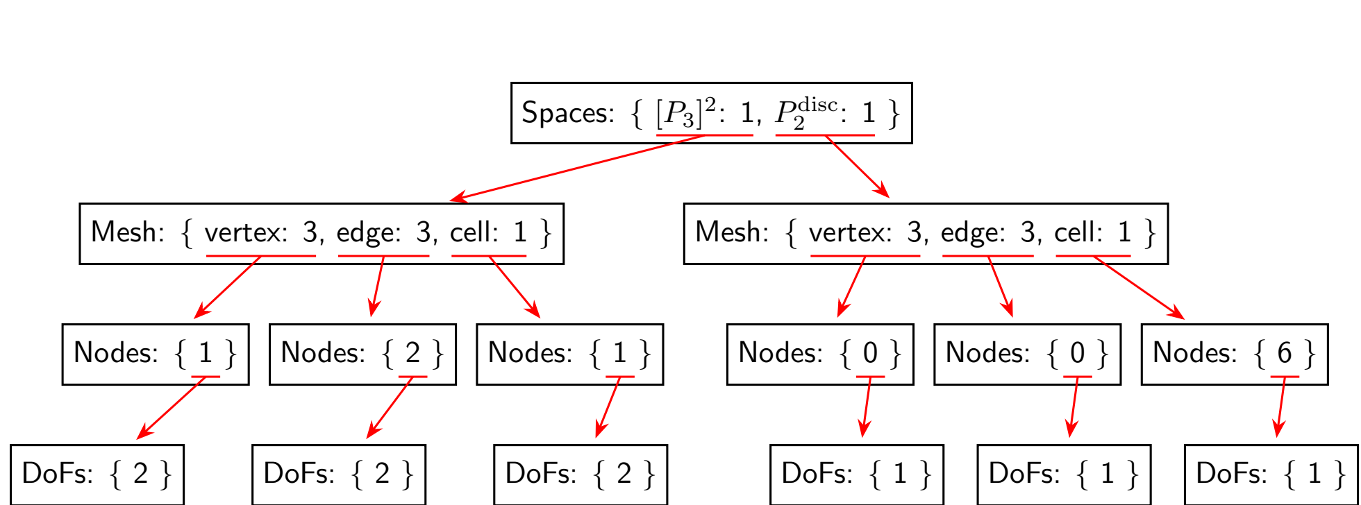
Figure 2: The data layout structure for a one-cell mesh of the finite element pair in fig. 1. It is not possible to capture all of this detail using an ND array.
