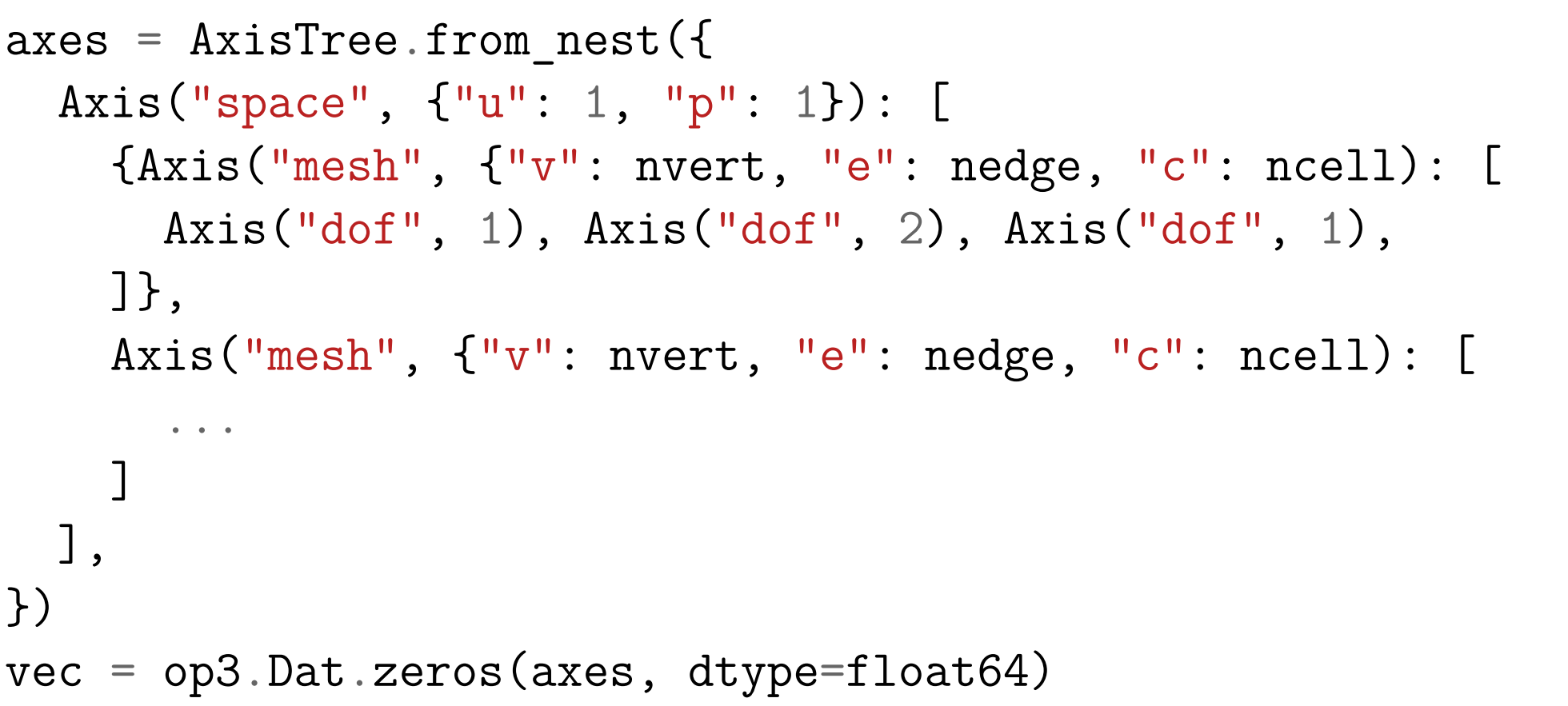
Figure 7: Simplified pyop3 code constructing a vector (termed a ‘dat’) with a data layout (axis tree) similar to that shown in fig. 3.
