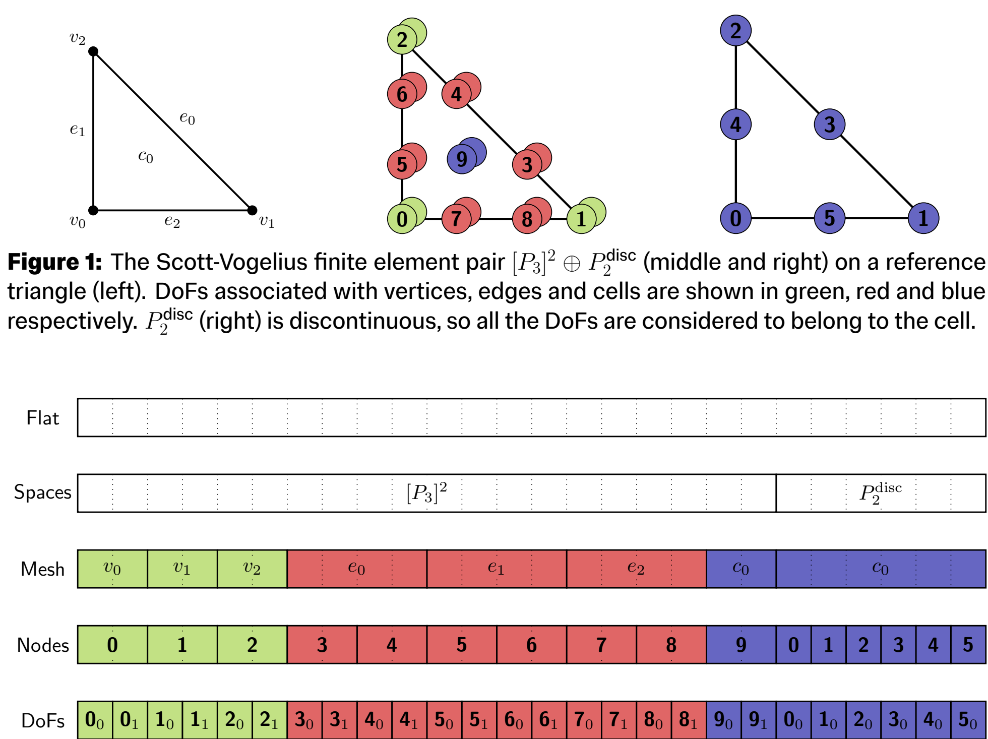
Figure 1: The Scott-Vogelius finite element pair [P_3]^2 \oplus P_2^{\text{disc}} (middle and right) on a reference triangle (left). DoFs associated with vertices, edges and cells are shown in green, red and blue respectively. P_2^{\text{disc}} (right) is discontinuous, so all the DoFs are considered to belong to the cell.
