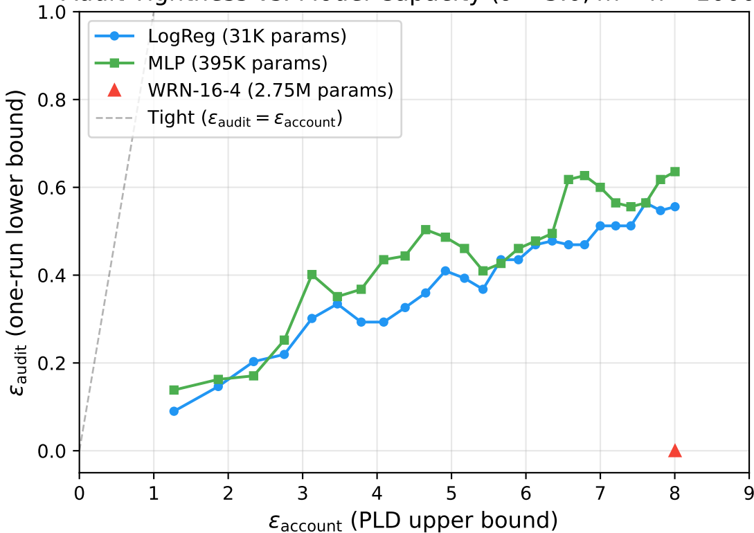
Audit Tightness vs. Model Capacity ( \sigma = 3.0 , m = n = 1000 )
