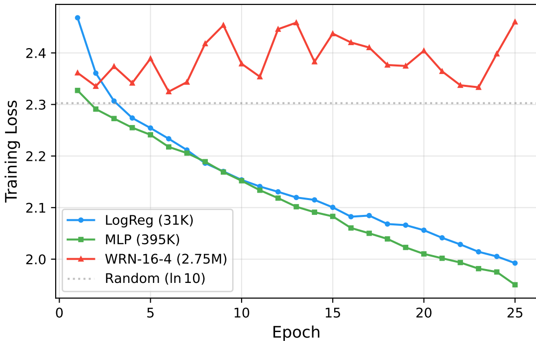
Training Loss Under DP-SGD ( \sigma = 3.0 , B = 500 )
