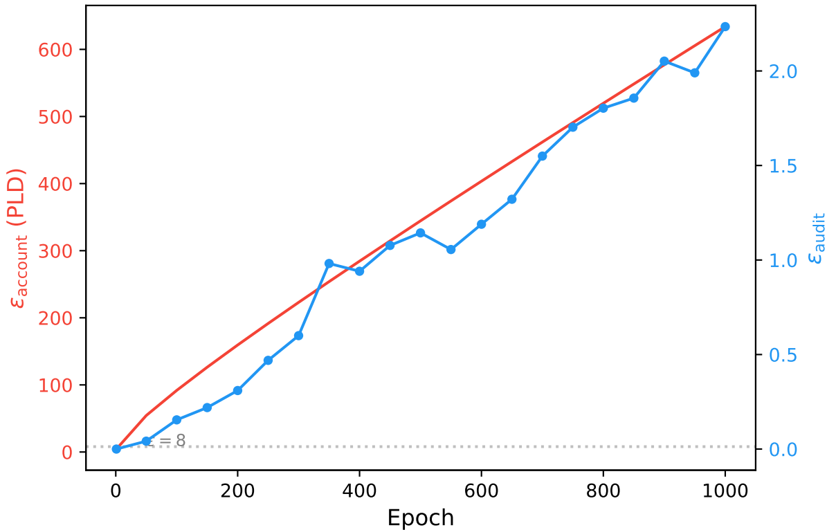
WRN-16-4: Audit Signal Requires Extended Training ( \sigma = 1.0 )
