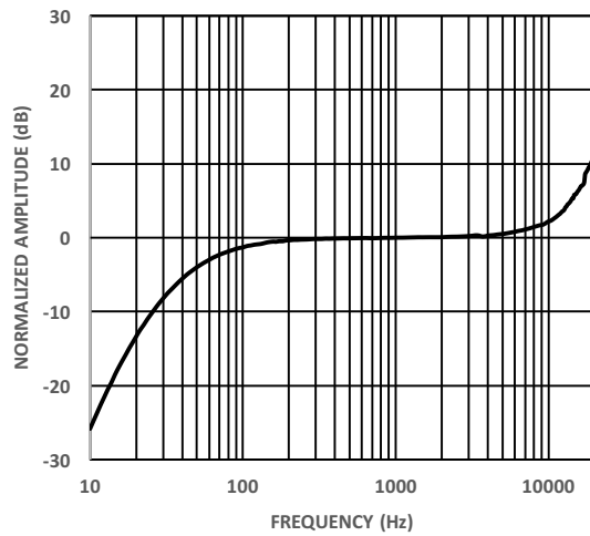
Figure 4. Typical Frequency Response (Measured)
