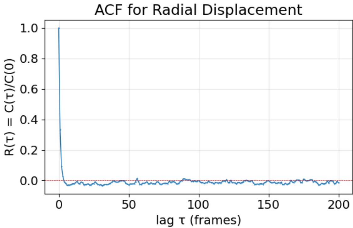
Figure 6.2: Slightly negative correlation in the bubble displacements, however fluctuates around zero mostly as expected
