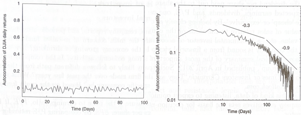
Figure 2.2: Dow Jones Industrial Average, autocorrelation of daily returns fluctuate around zero, autocorrelation of the volatility follows a power law.
