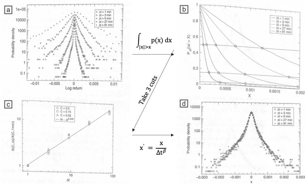
Figure 2.3: Series of figures which describes how complementary cumulative distribution functions can be use to collapse data onto a master plot. [2]
