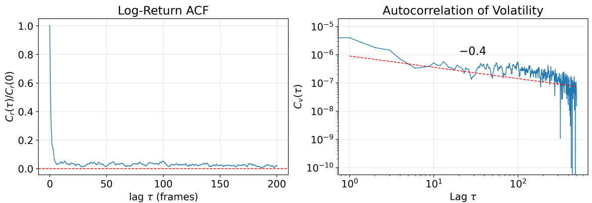
Figure 4.12: Log return ACF unexpectedly stays ever so slightly positive, the volatility ACF follows a power law trend that can be linked back to the DJIA figure 2.2.
