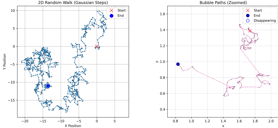
Figure 4.2: Comparison of a Brownian random walk (left) and a tracked bubble path (right) over the same number of timesteps.
