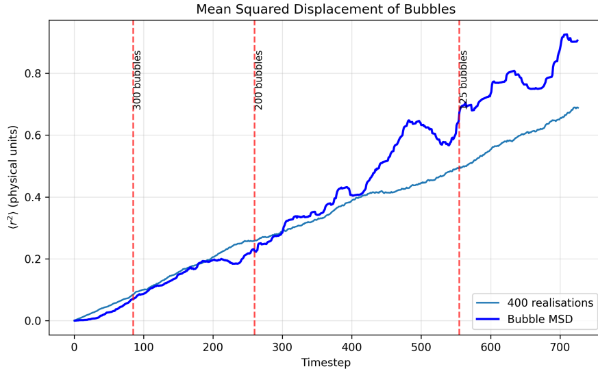
Figure 4.4: Mean squared displacement for the bubble data with the MSD for 400 Brownian walks overlayed to compare linearity.
