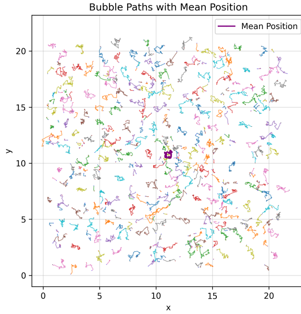
Figure 4.1: Paths of the centres of the bubbles.
