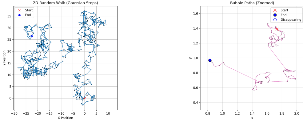
Figure 4.2: Comparison of a Brownian random walk (left) and a tracked bubble path (right) over the same number of timesteps.
