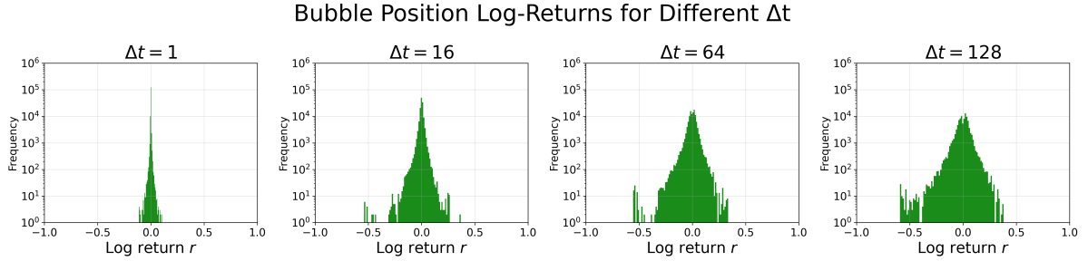
Figure 4.6: Log return distributions over increasing \Delta t . Distribution does not widen into a Gaussian unlike the displacement distributions. Log-linear scale.
