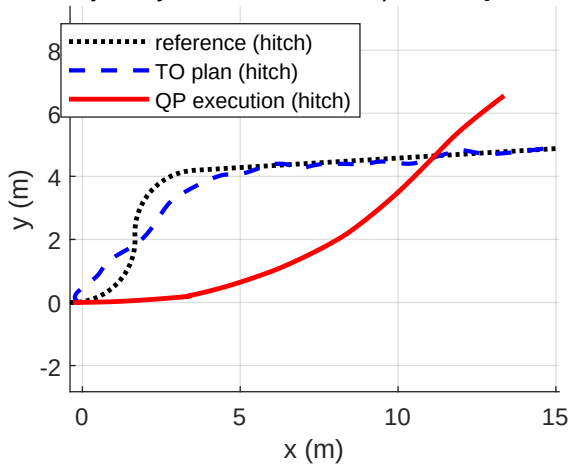
hitch trajectory: reference vs TO plan vs QP execution
