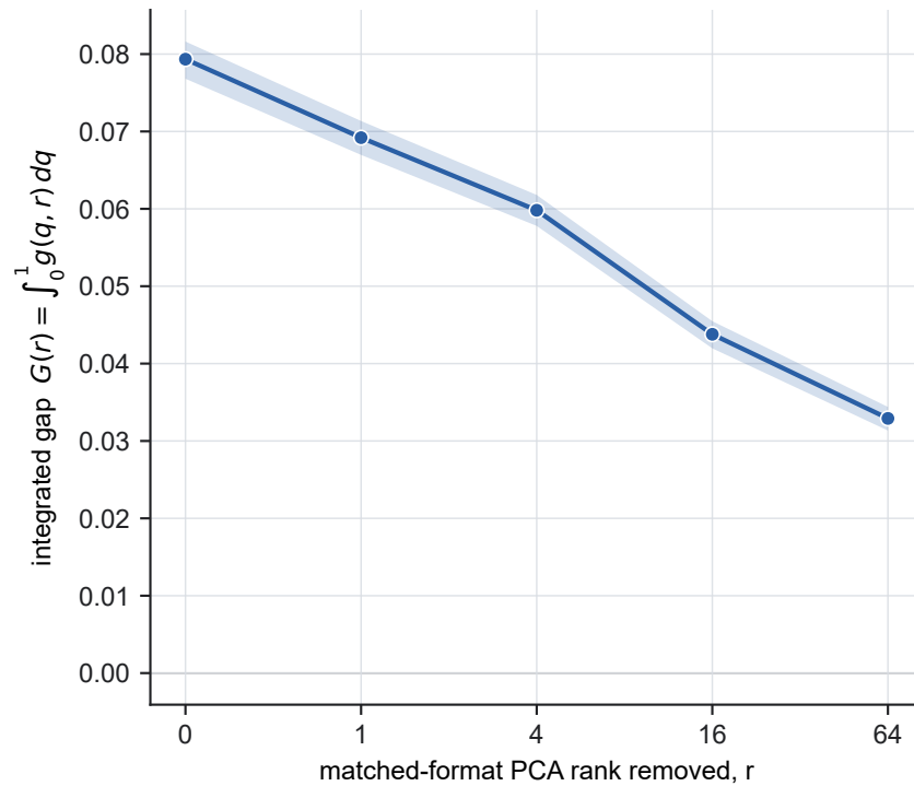
Integrated gap vs. rank
