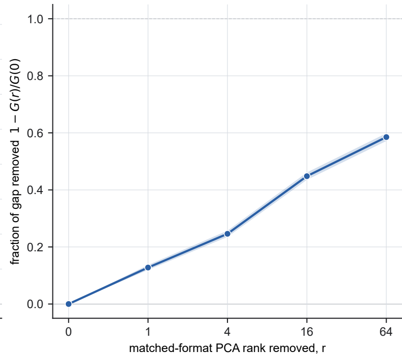
Fraction removed vs. rank
