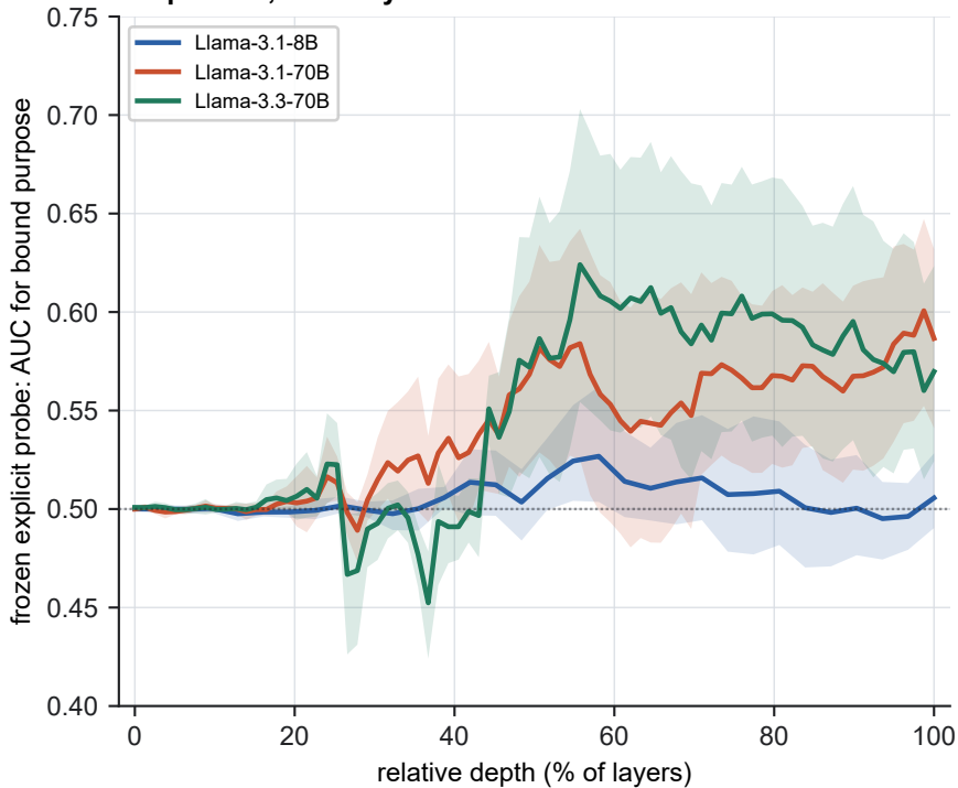
A. Frozen explicit purpose probe transfers only in the deeper half, and only at 70B scale
