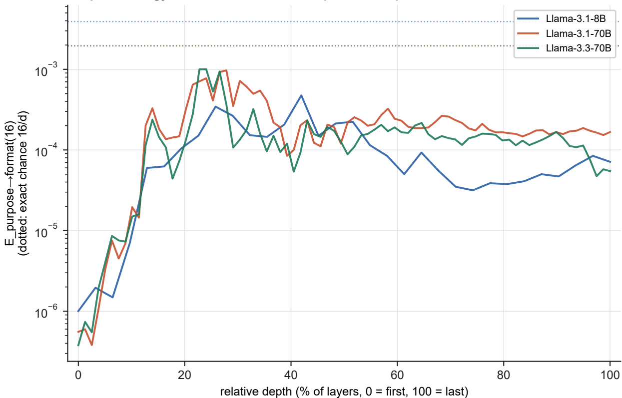
Purpose energy in matched-format subspace vs. depth
